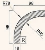
R78 – NỆP CONG R78
